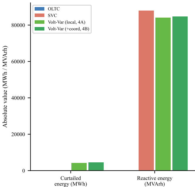
(B) Absolute -- RPi HIL Dry
