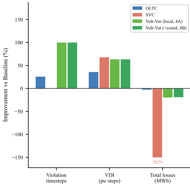
(A) % Improvement -- RPi HIL Dry
